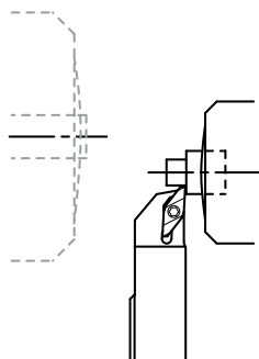
TURN-Line ISO-Line
